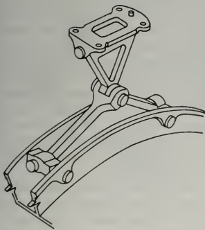
B. Aft mount
